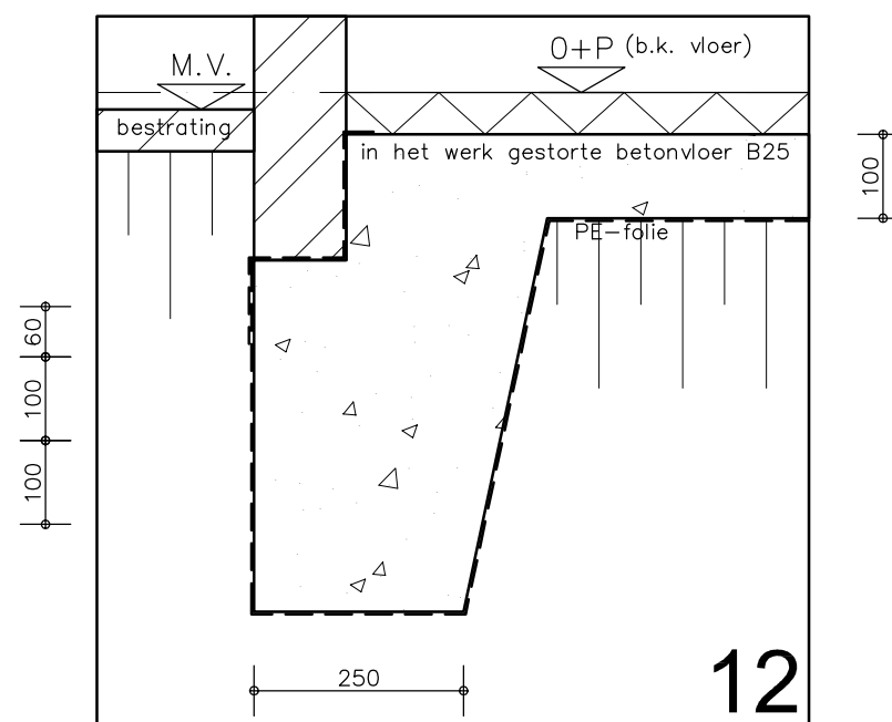
detail fundering berging
