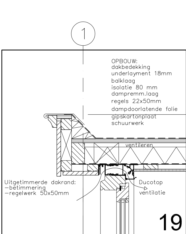
detail dakrand dakkapel
