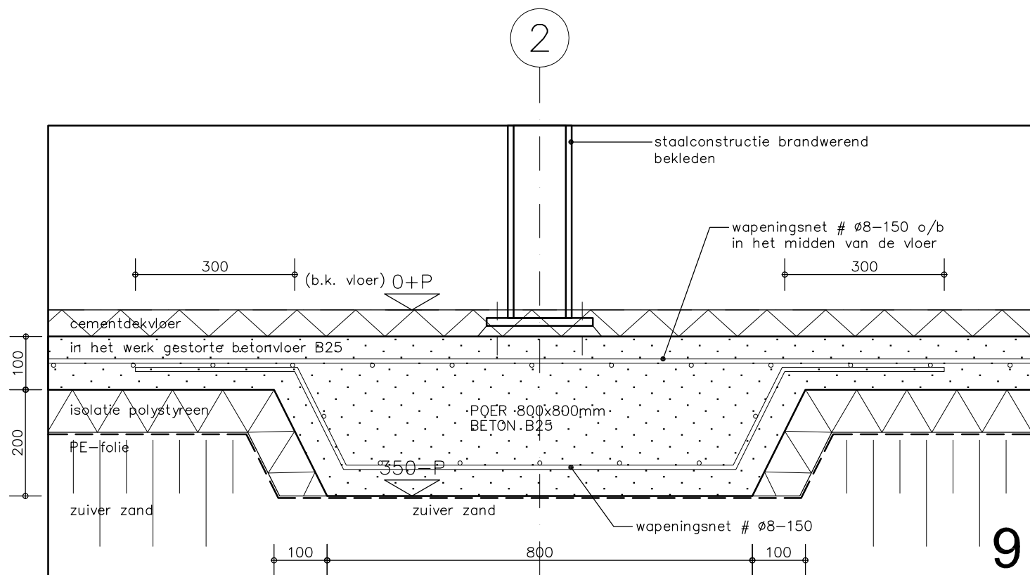
detail poer-fundering
